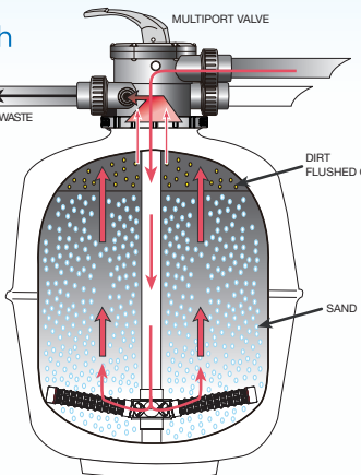
Backwash Mode
