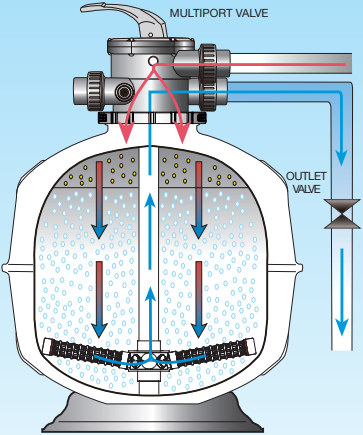
Backwash Mode
