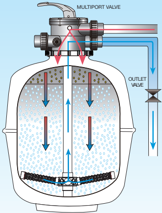
Filter Mode
