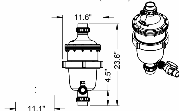
MULTICYCLONE 16 (200370)
