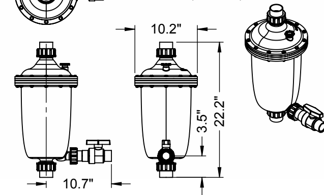
MULTICYCLONE 12 (200371)
