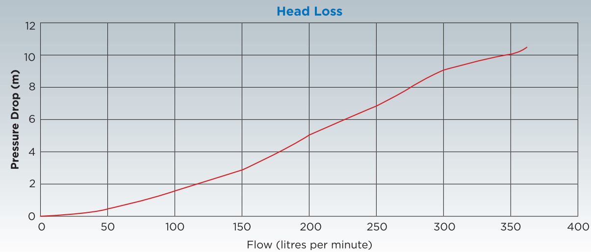
MULTICYCLONE 16 (200370)
