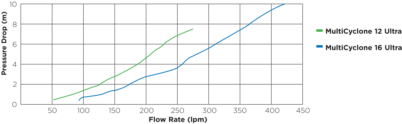
Head Loss Curves
