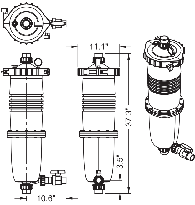
MultiCyclone 12 Ultra
